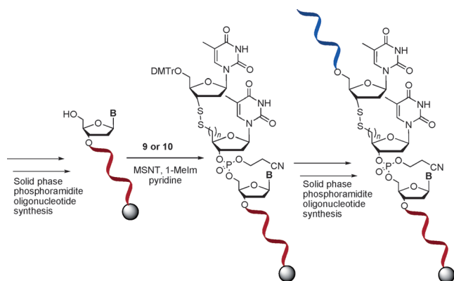
Scheme 2. Oligonucleotide synthesis employing a mixed phosphoramidite and phosphotriester strategy for the incorporation of disulfide dithymidines 16 and 17 . MSNT = 1-(2-mesitylsulfonyl)-3-nitro-1H-1,2,4-triazol; 1-Melm = 1-methylimidazole.
